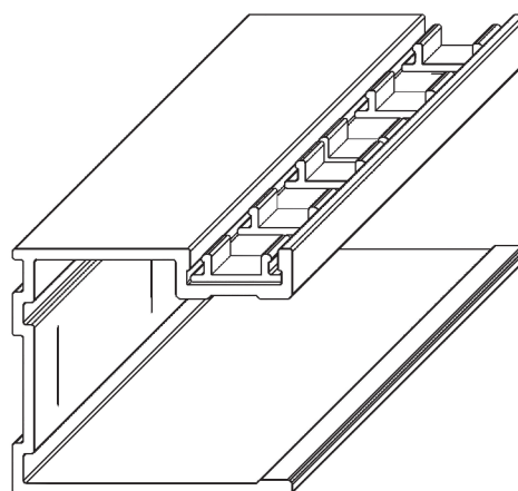
Wall Profile & Cover Clip Sub Assy x1
