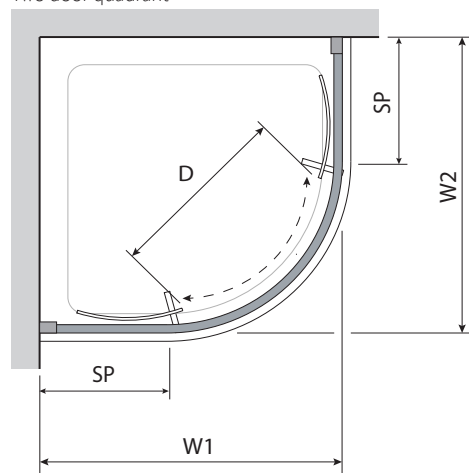
Two door offset quadrant
