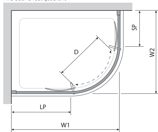
Two door offset quadrant
