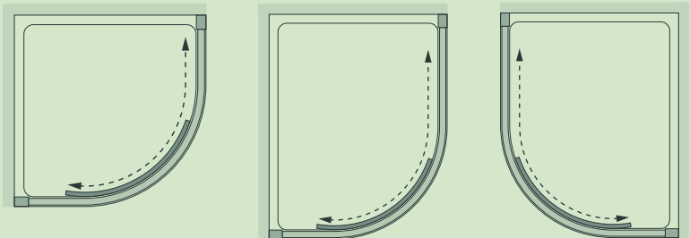
Single Door Quadrant Offset Left-Hand Tray Offset Right-Hand Tray
