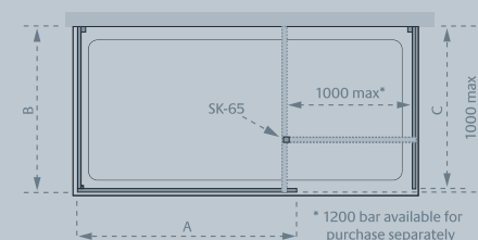
Shower Panel, End Panel &amp; Side Panel
