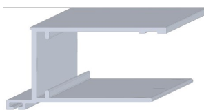
Vertical Frame Rail (door side) (1950mm 1x)
