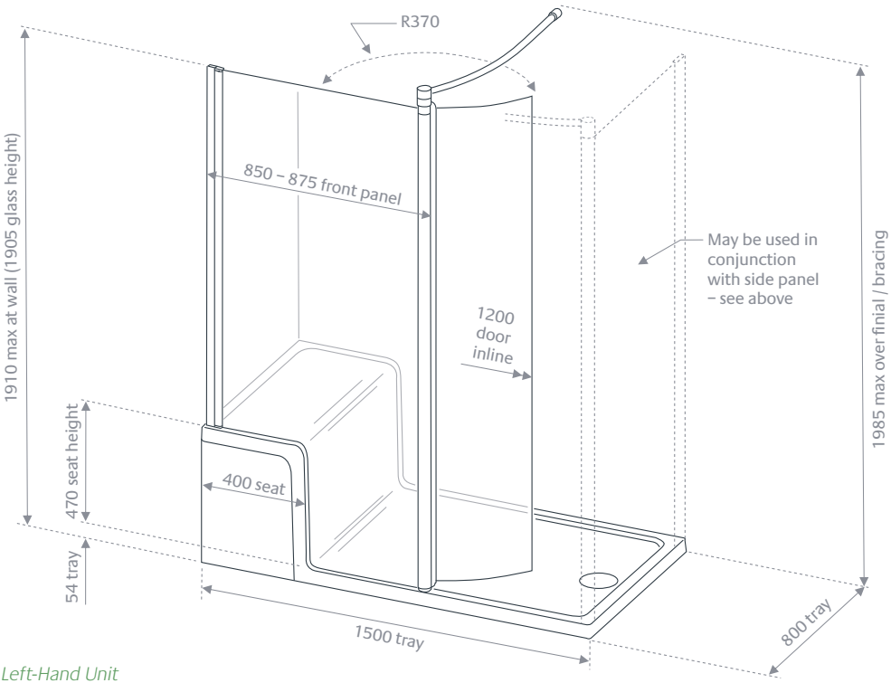
Left-Hand Unit
